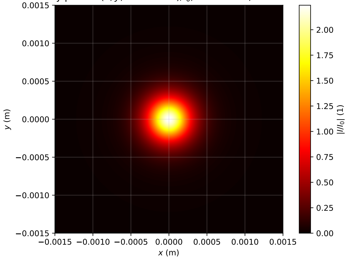
Intensity profile I(x, y, z = 2.229m)/I_0 , P_{in}=1.0P_{cr} , artificial time
